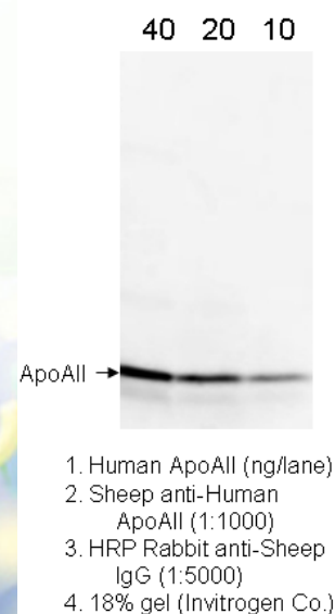
Western Blot Data for Affinity Purified Sheep Anti-Human ApoAII Antibody
